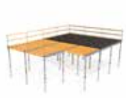
Drophead slab shoring
